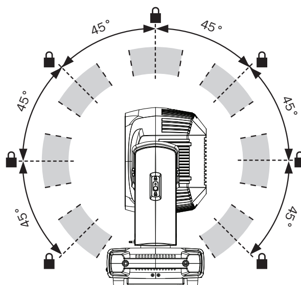
Tilt mechanism lock and release every 45°
